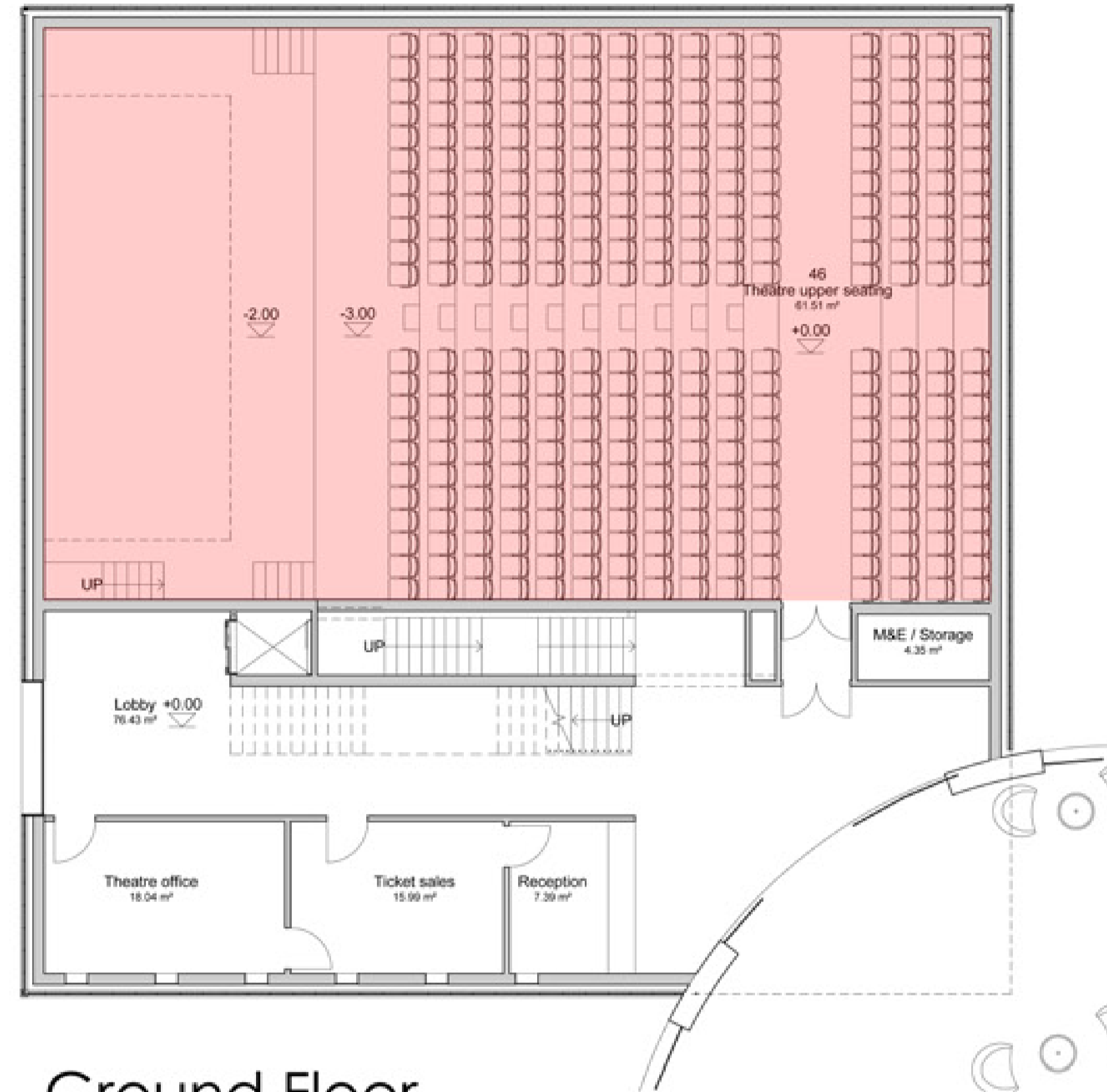
Ground Floor
