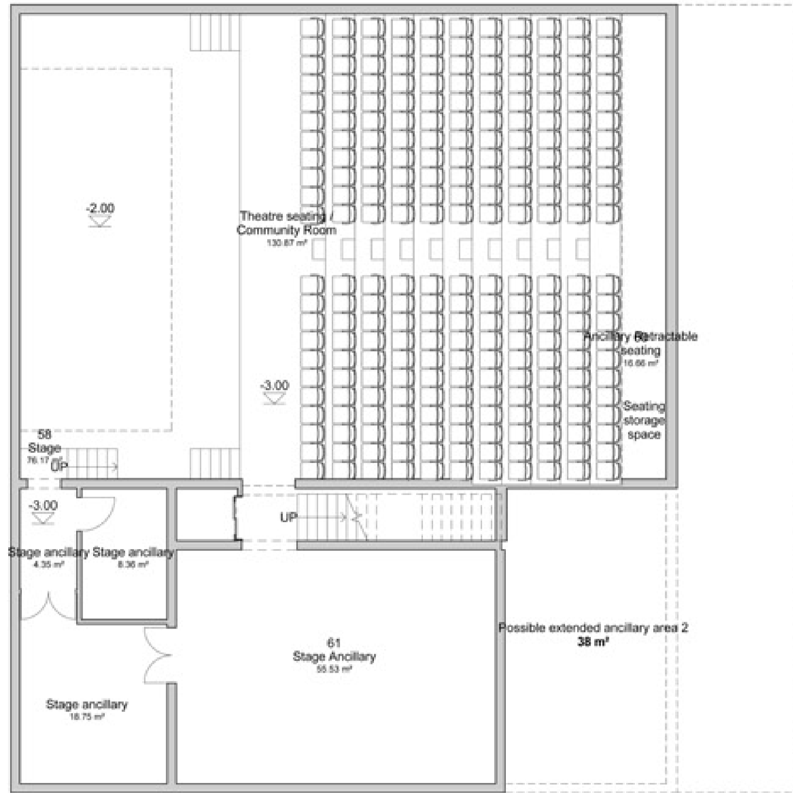
Level -1
