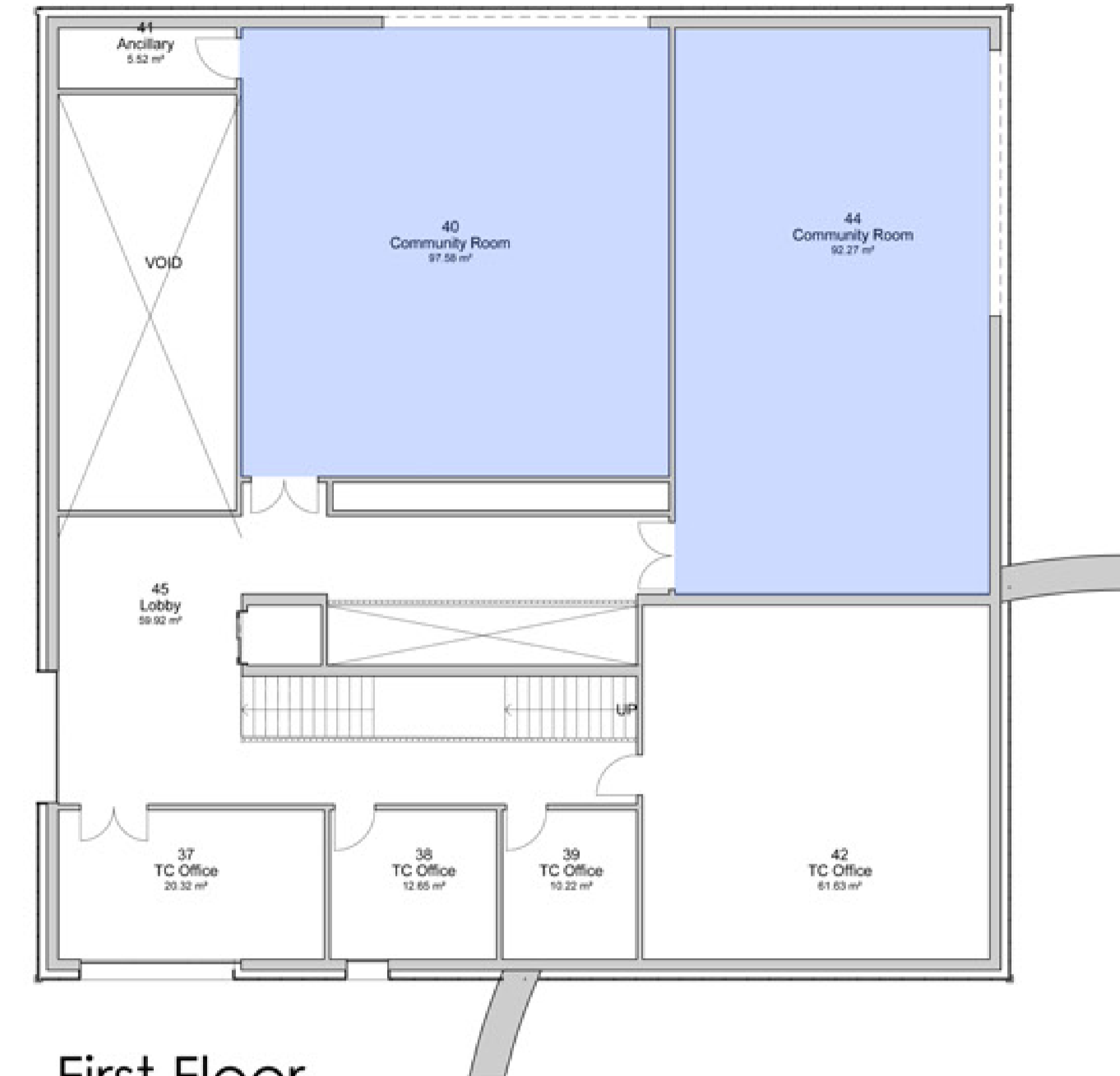
First Floor
